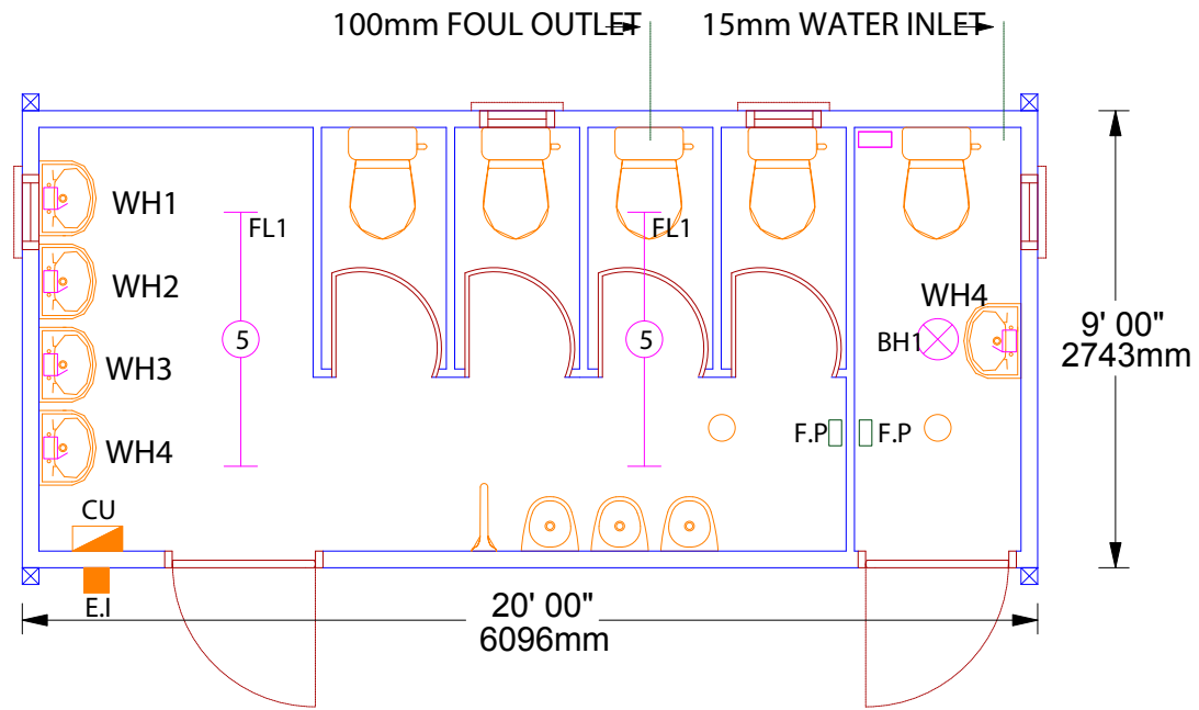
20' x 9' 4+1 TOILET
