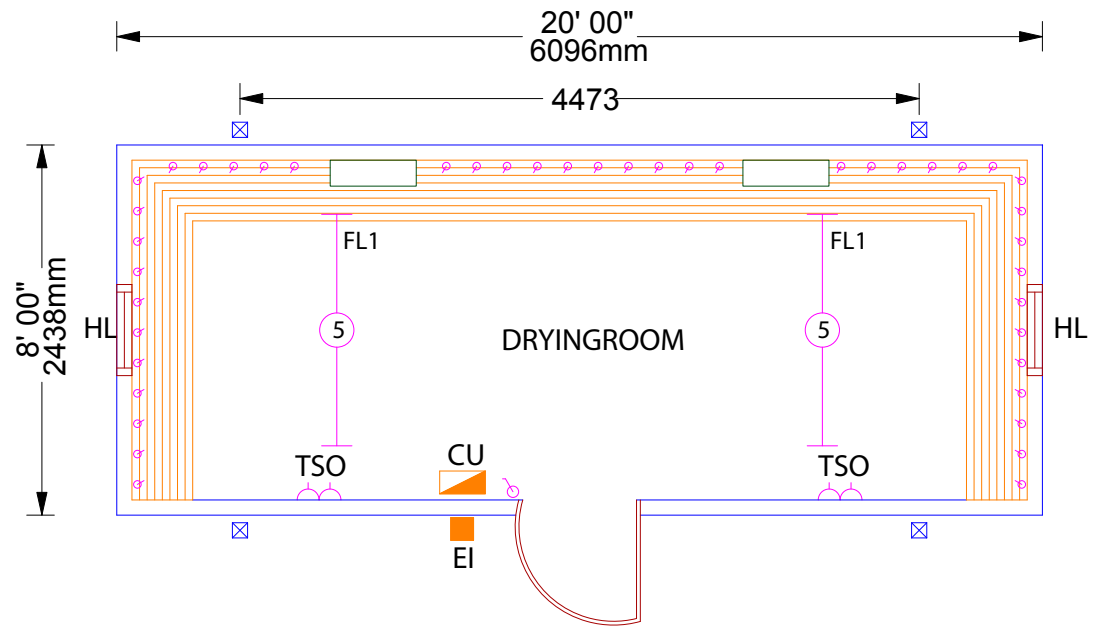
20' x 8' DRYINGROOM
